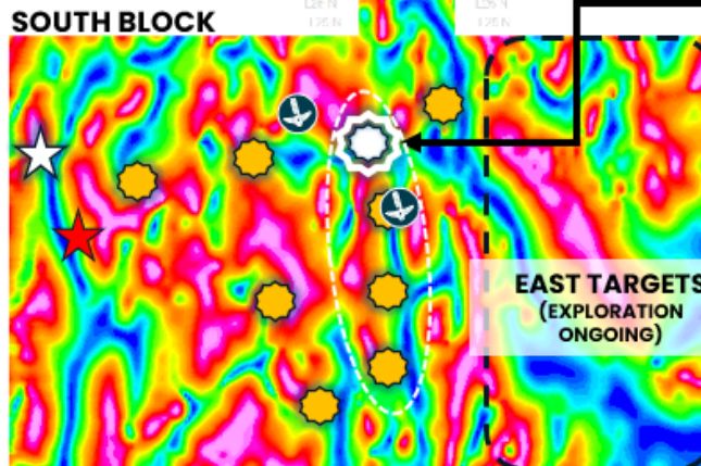
Figure 1. Gran Pilar target summary. Drone magnetic survey map showing tilt derivative of the Reduced to Pole (RTP) and priority target areas identified to date by geological mapping and surface geochemistry. Location of the new El Mezquite target area.
