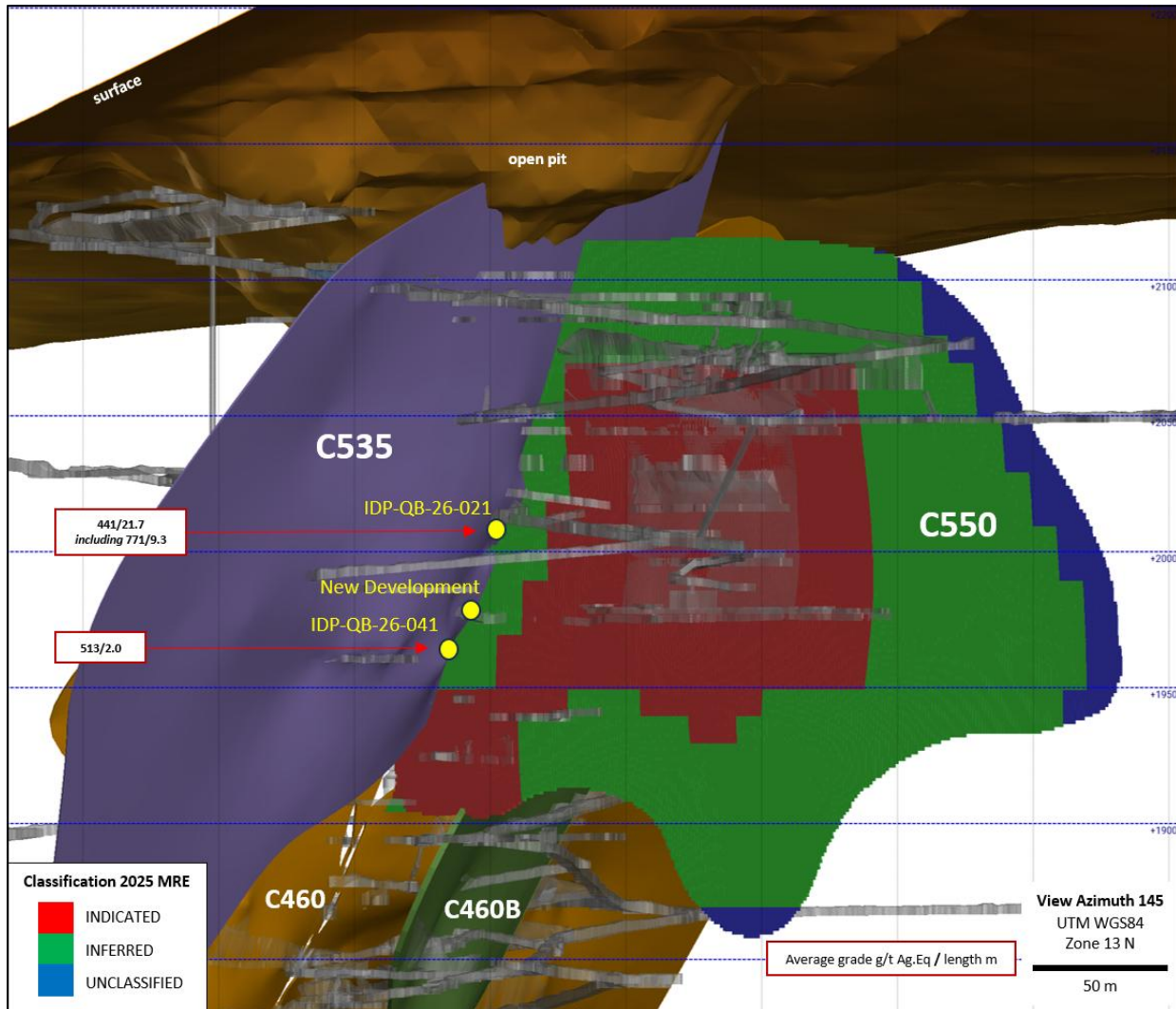
Figure 2: Cross section view of the C550 and C535 Zones
