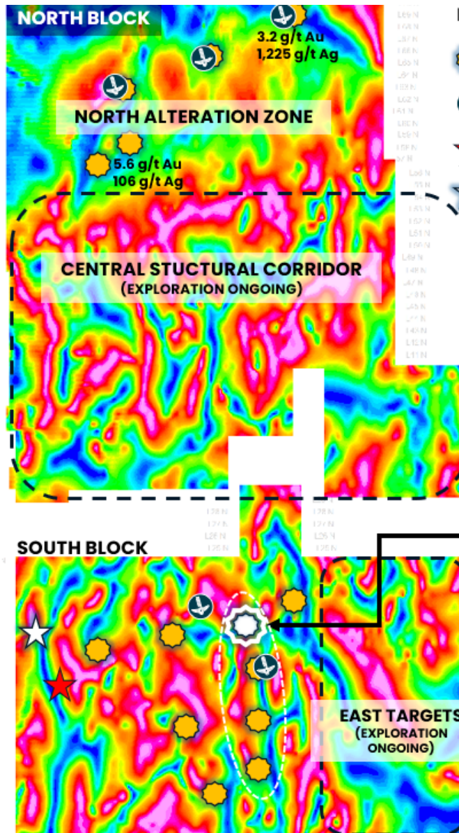
Figure 2. Gran Pilar target summary. Drone magnetic survey map showing tilt derivative of the Reduced to Pole (RTP) and priority target areas identified to date by geological mapping and surface geochemistry. Location of the new El Mezquite target area.
