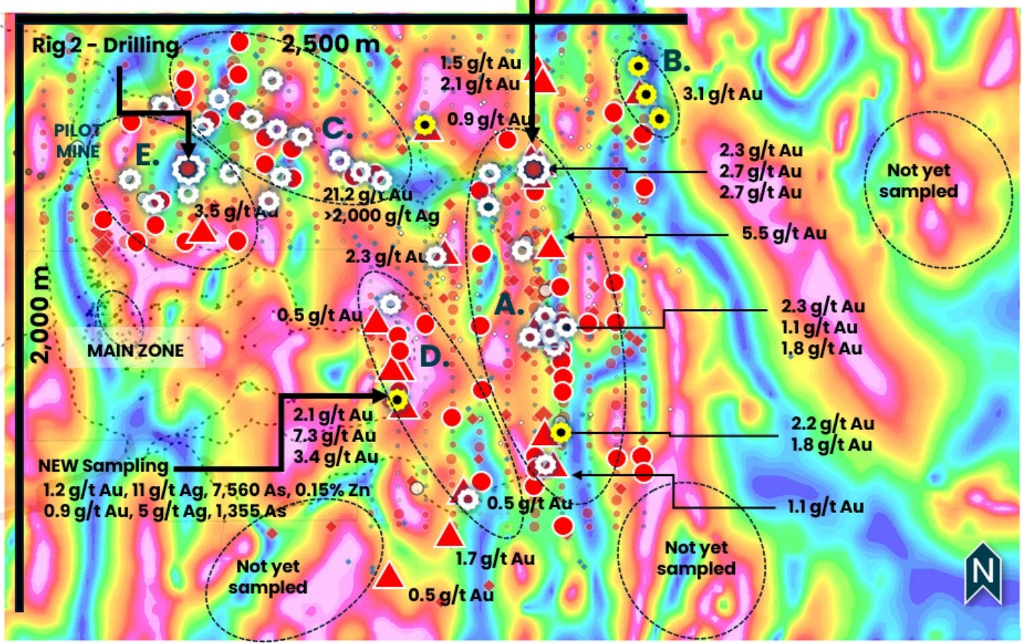
Figure 1. Current drill targets within the South Block. Drone magnetic survey map showing tilt derivative of the Reduced to Pole (RTP) and priority target areas identified to date by geological mapping and surface geochemistry. Location of the new El Mezquite target area.
