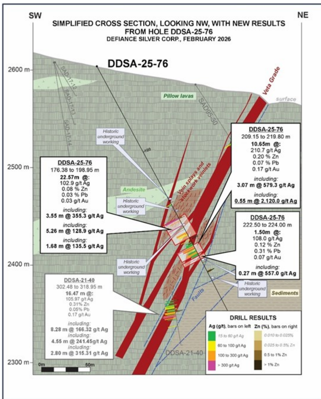
Figure 2. Simplified Cross Section, looking NW with results from Hole DDSA-25-76
