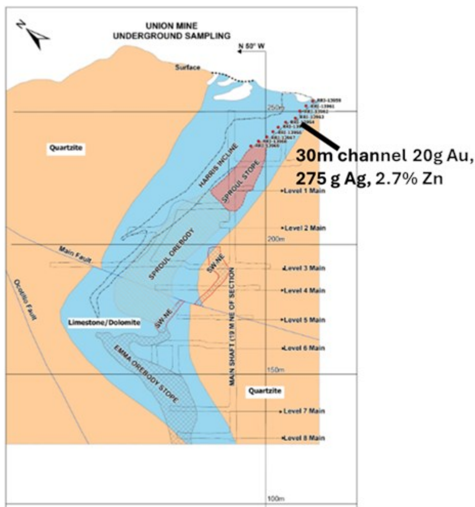
Figure 2: Cross section of the Union underground sampling and some of the orebodies previously mined that could have remaining potential as CRD targets for next round of follow up.
