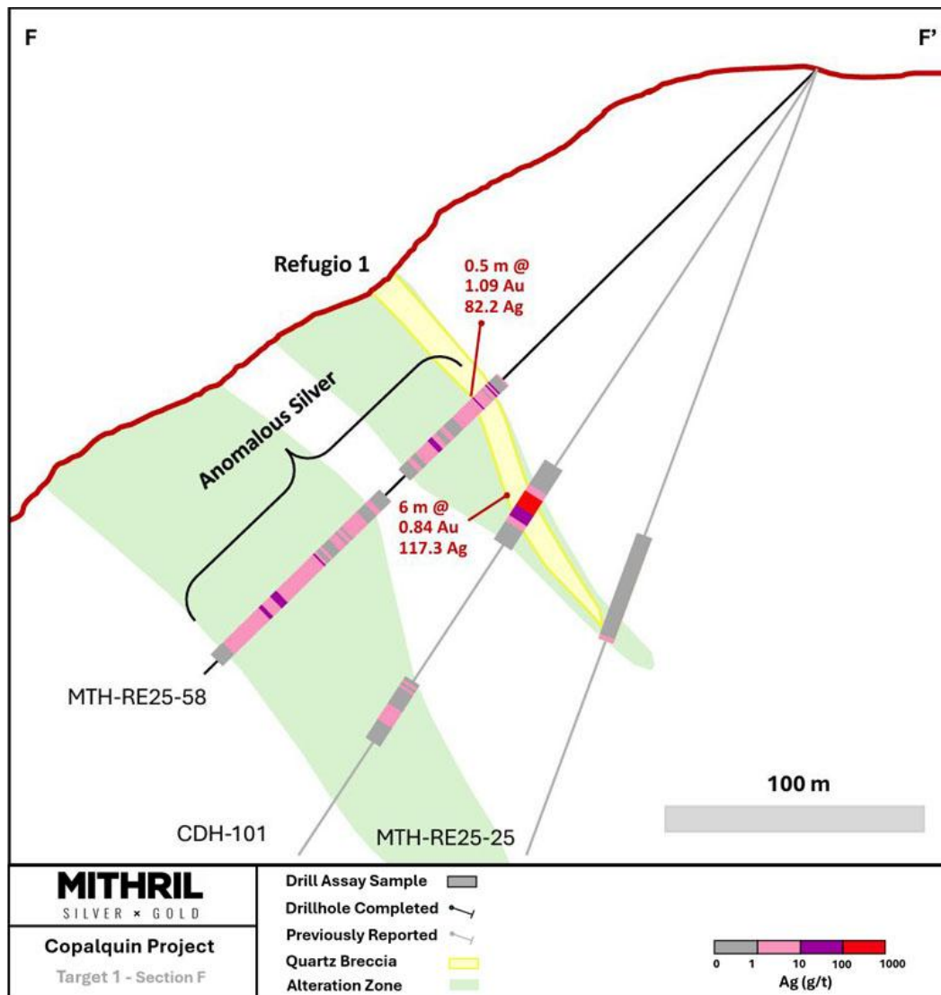
Figure 7 Drill hole MTH-RE25-58 intercepted a thick anomalously silver rich alteration halo on the western side of Target 1
