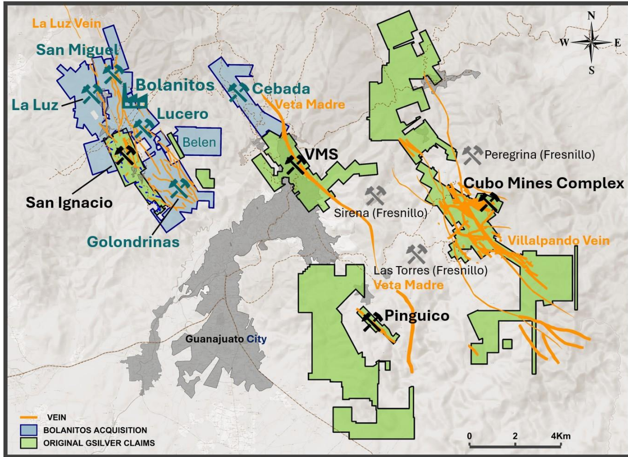
Figure 1: Map of the Guanajuato Mining District showing the main epithermal veins and other significant geological structures. Bolanitos is located along the La Luz Vein structure.
