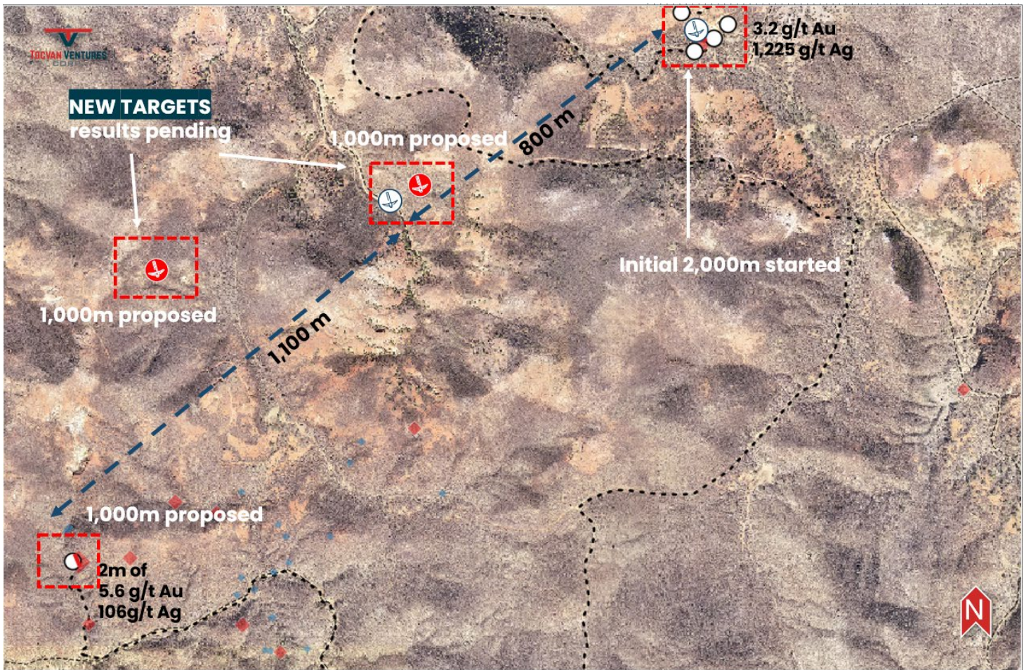
Figure 1. Map of North Alteration Zone with key target areas within alteration footprint. Drilling has started on the northern most target. Mapping and sampling in the central location is ongoing, with results pending.
