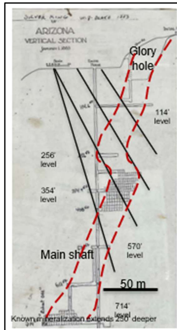
Figure 2. Cross section through the Silver King mine workings showing proposed drill holes (in black) to test the pipelike mineralized body (in red)
