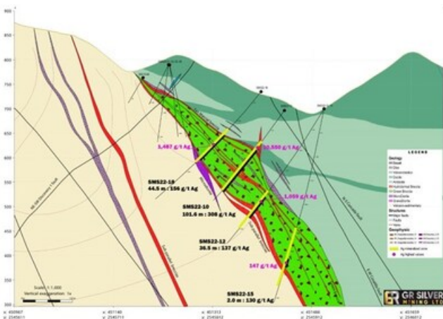
Figure 2: Geological Section A-B, SE Discovery Area, delineation of a wide, mineralized silver zone (CNW Group/GR Silver Mining Ltd.)
