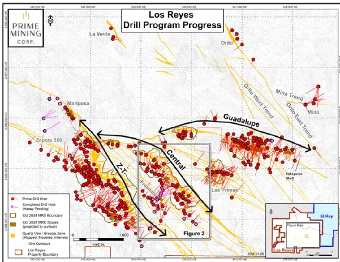
Central Drill Hole Highlights 1
