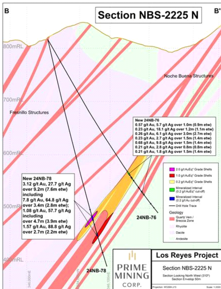
Figure 4: Central Trend (Noche Buena) cross section B-B'
