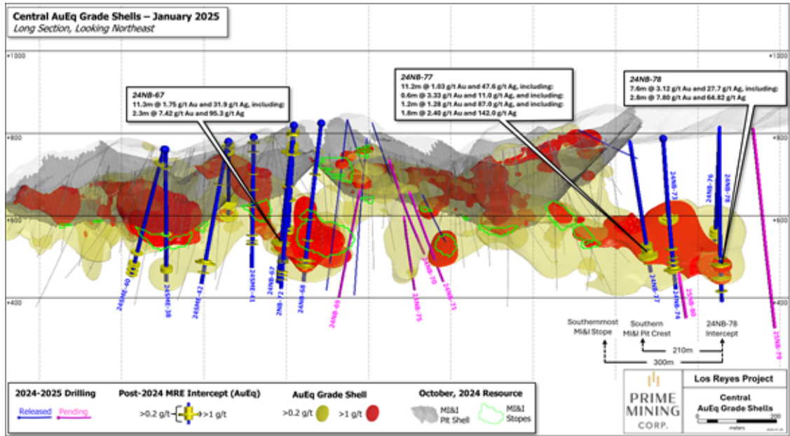
Figure 3: Central Trend long section with drill holes highlighted (A-A')
