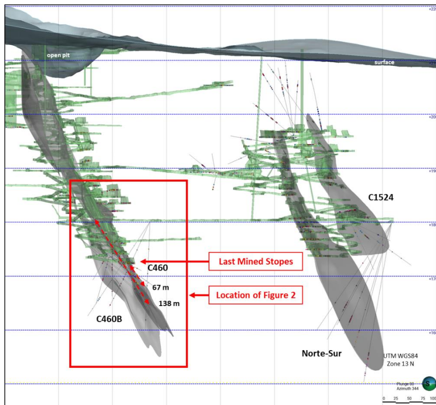
Figure 1: Cross Section of Quebradillas Mine View Towards NNW
