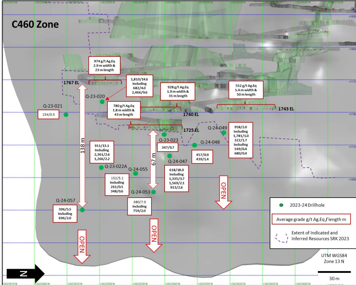
Figure 2: Longitudinal Section of C460 Zone View Towards West
