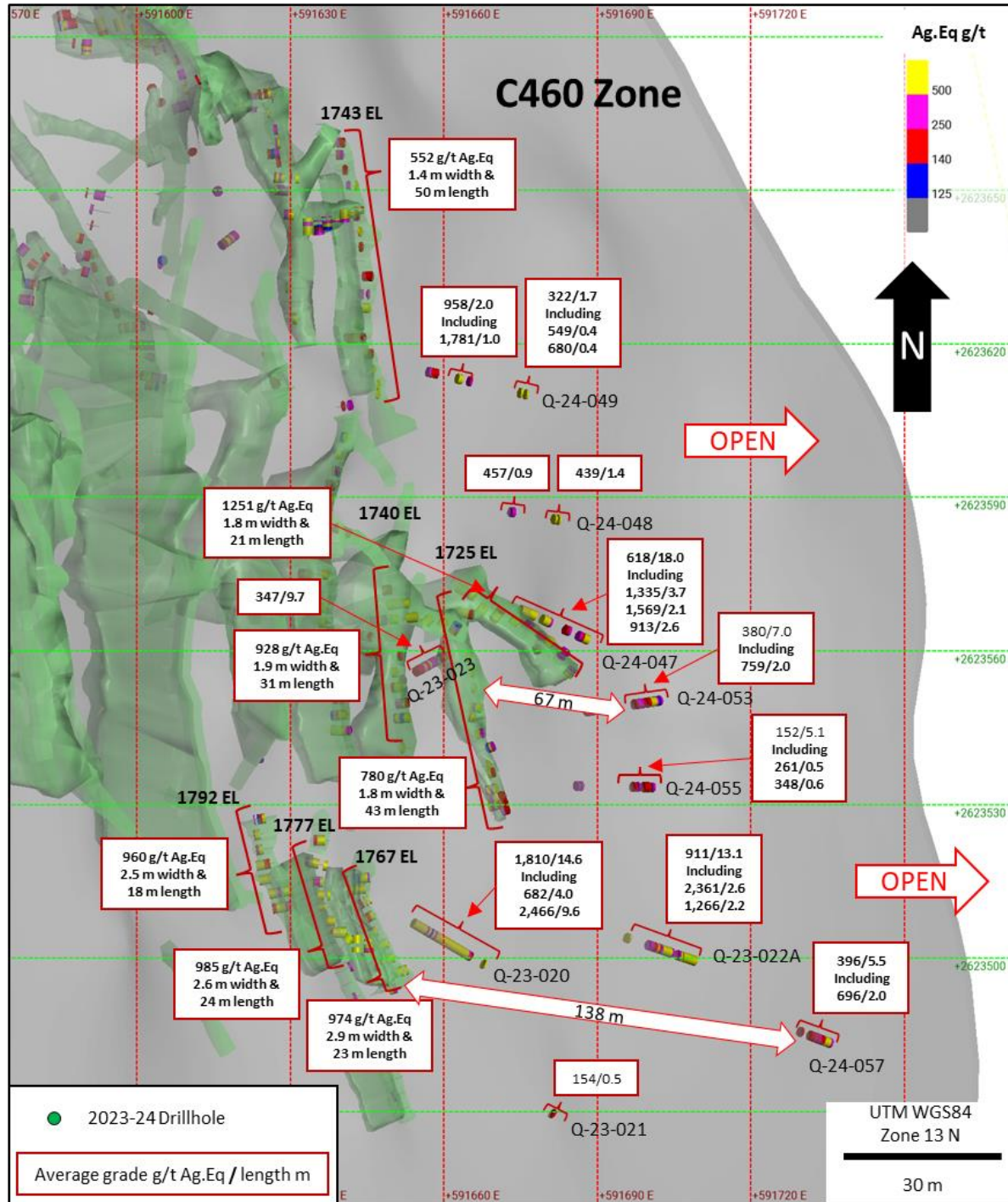
Figure 3: Plan View of C460 Zone 1800 EL and Below
