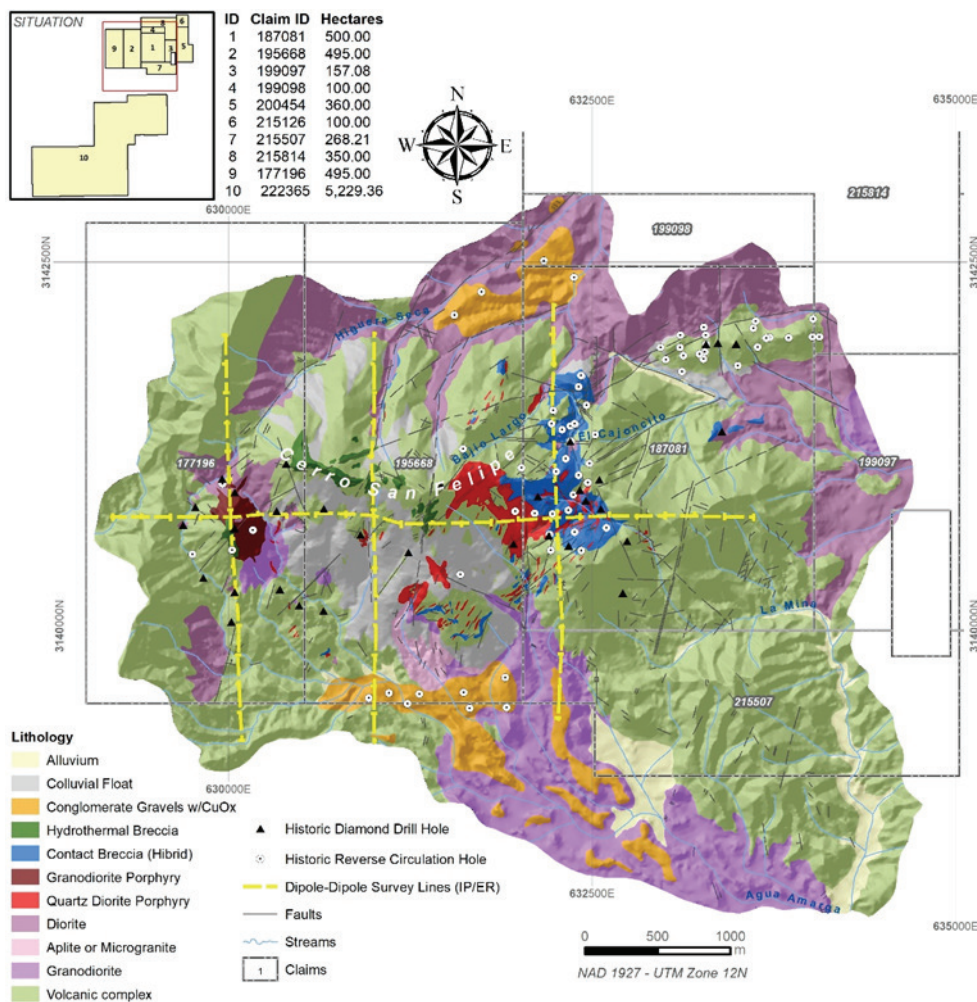
Figure 1 shows the geological map and arrangement of the historical data in the project areas.
