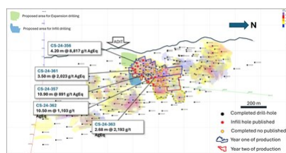
Figure 2. Longitudinal section of Copala vein with mineral resources, planned stopes, drill-hole intercepts and location of the recently discovered Copala adit. (CNW Group/Vizsla Silver Corp.)
