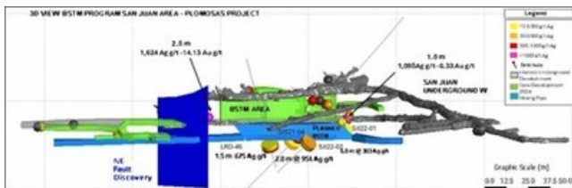
Figure 1 - Lay Out Bulk Sampling Trial Mining (‘BSTM’): Underground Development - San Juan Area (CNW Group/GR Silver Mining Ltd.)
