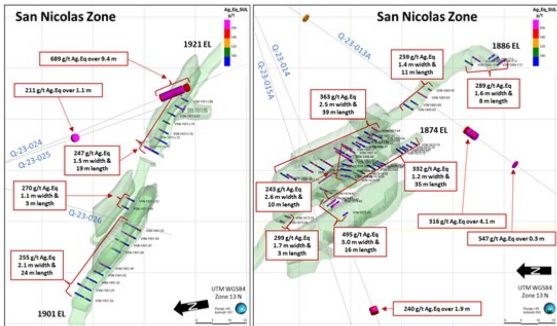
Figure 3: Oblique View to East of San Nicolas Channel Samples 1874, 1886, 1901 & 1921 m EL Stopes
