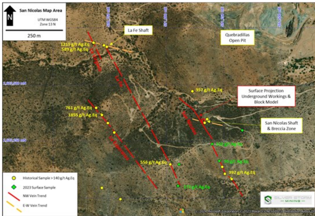
Figure 5: Surface Plan of San Nicolas, La Fe, La Virginia, & La Esperanza Zones
