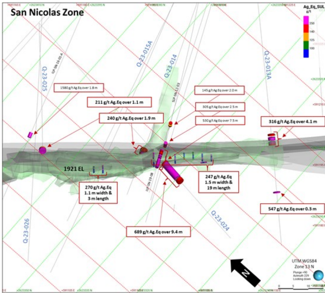
Figure 2: Plan View San Nicolas Zone
