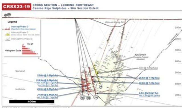
Figure 3: Camino Rojo Cross Section Drill Intersection Highlights for Fence CRSX23-19 (CNW Group/Orla Mining Ltd.)
