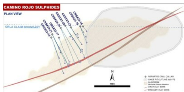
Figure 1: Plan View Showing Location of Reported Drill Holes (CNW Group/Orla Mining Ltd.)
