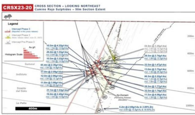
Figure 4: Camino Rojo Cross Section Drill Intersection Highlights for Fence CRSX23-20 (CNW Group/Orla Mining Ltd.)
