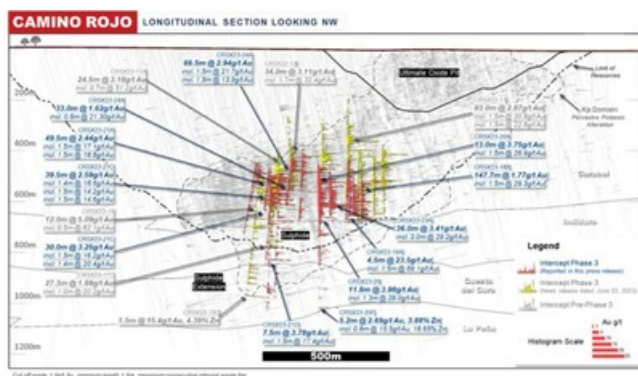
Figure 2: Camino Rojo Long Section Drill Intersection Highlights (CNW Group/Orla Mining Ltd.)
