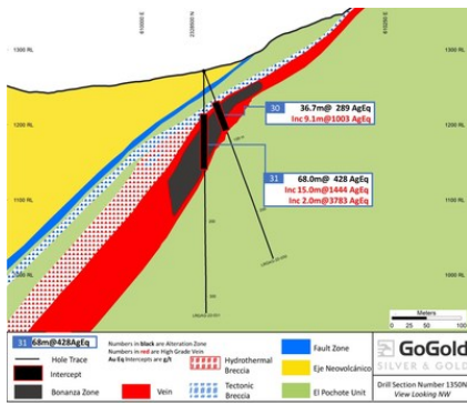
Figure 2: Eagle – Cross Section Holes 30,31 (CNW Group/GoGold Resources Inc.)
