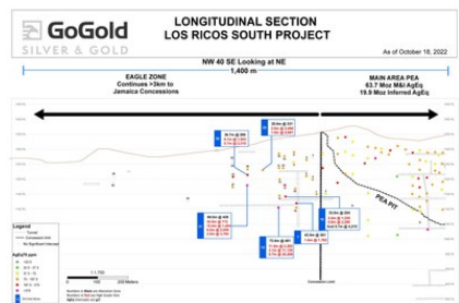
Figure 5: Eagle Longitudinal Section (CNW Group/GoGold Resources Inc.)
