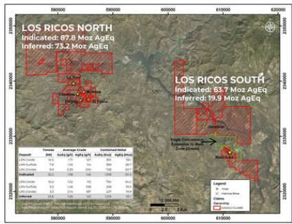
Figure 6: Los Ricos District Overview (CNW Group/GoGold Resources Inc.)
