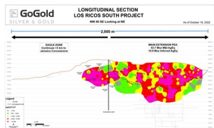
Figure 4: Eagle + Main Area Longitudinal Section (CNW Group/GoGold Resources Inc.)
