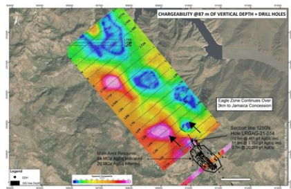
Figure 3: Eagle & Main Area Geophysics (CNW Group/GoGold Resources Inc.)
