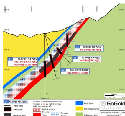
Figure 1: Eagle – Cross Section Holes 11, 12, 13, 14 (CNW Group/GoGold Resources Inc.)
