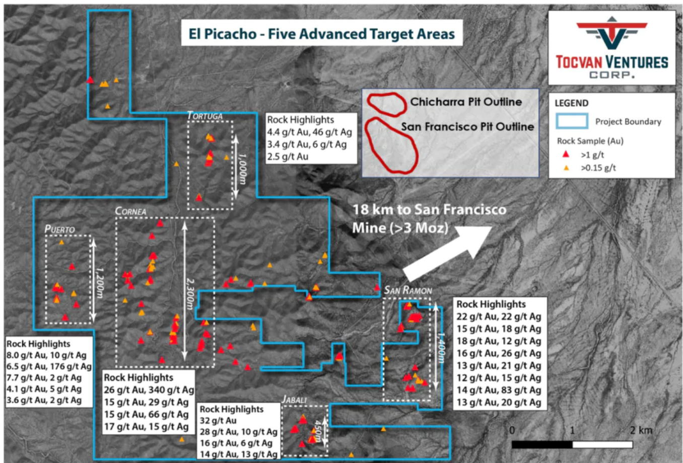
Figure 5. Overview map of the El Picacho Gold-Silver Project
