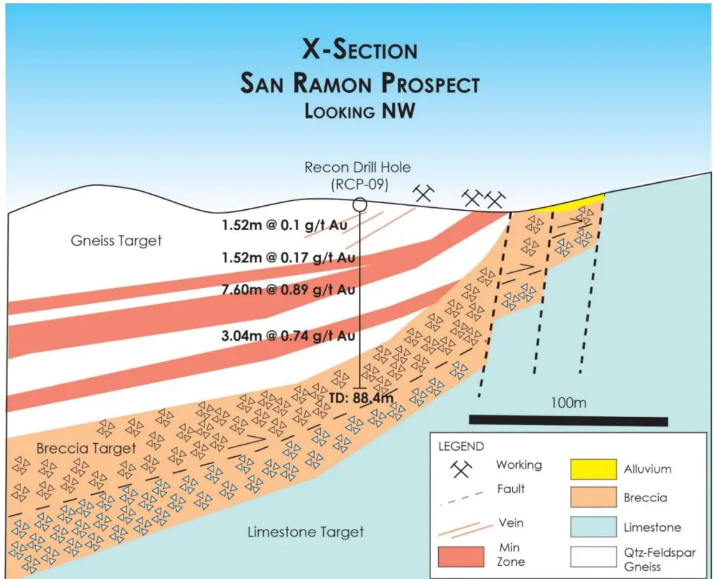
Figure 3. X-Section of the San Ramon Prospect and Drill hole RCP-09. The drill hole was lost at 88.4-meters, failing to test the lower sediment host target horizon.
