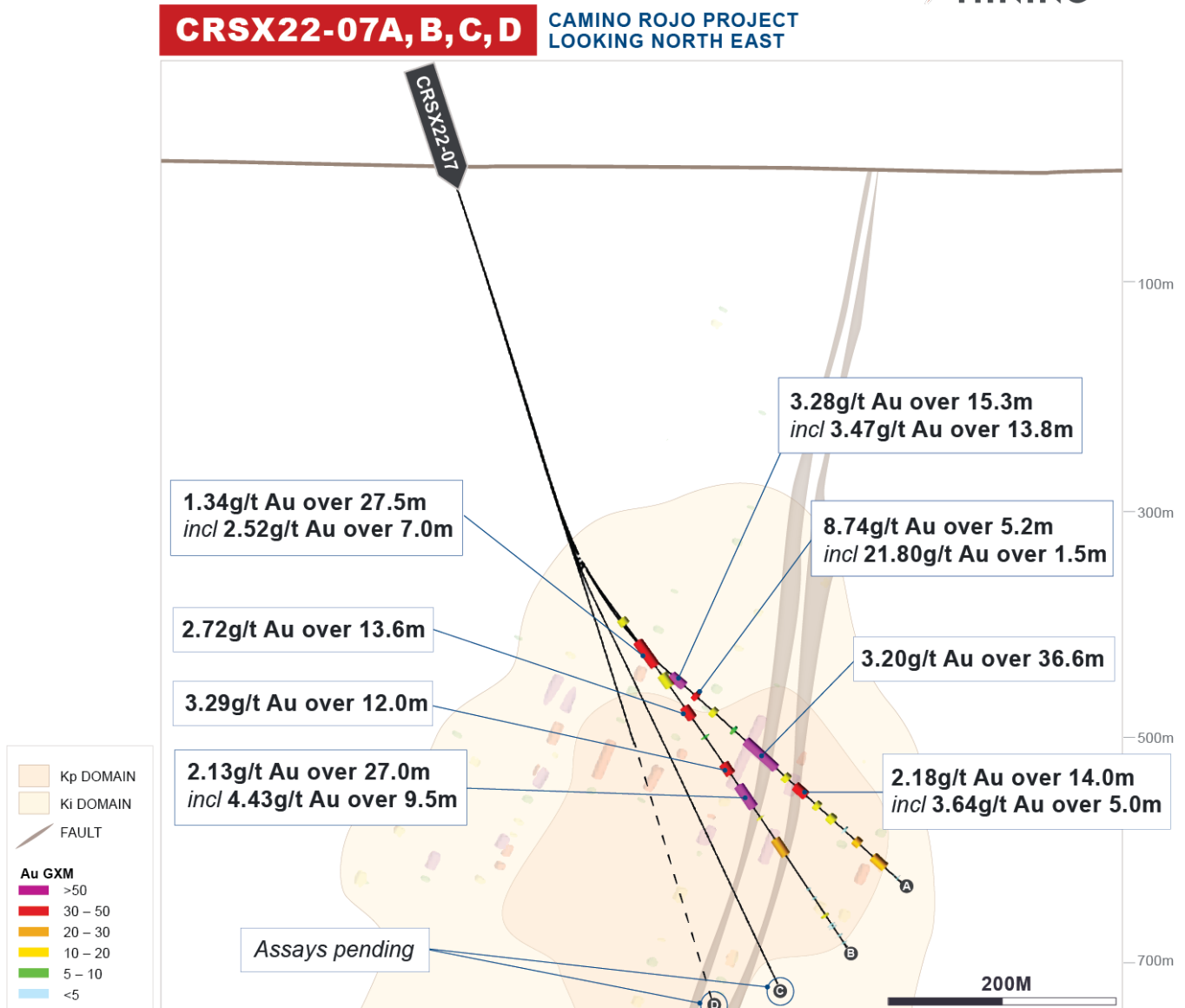
Figure 3: Camino Rojo Sulphides Cross Section (CRSX22-07)
