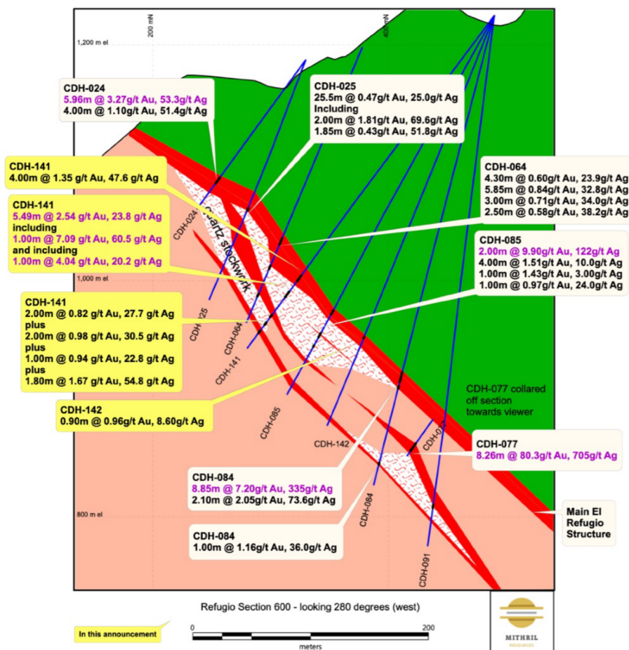
Figure 2 – Cross section 600 showing the well developed El Refugio structure which hosts multiple gold-silver bearing veins including very high-grade grades
