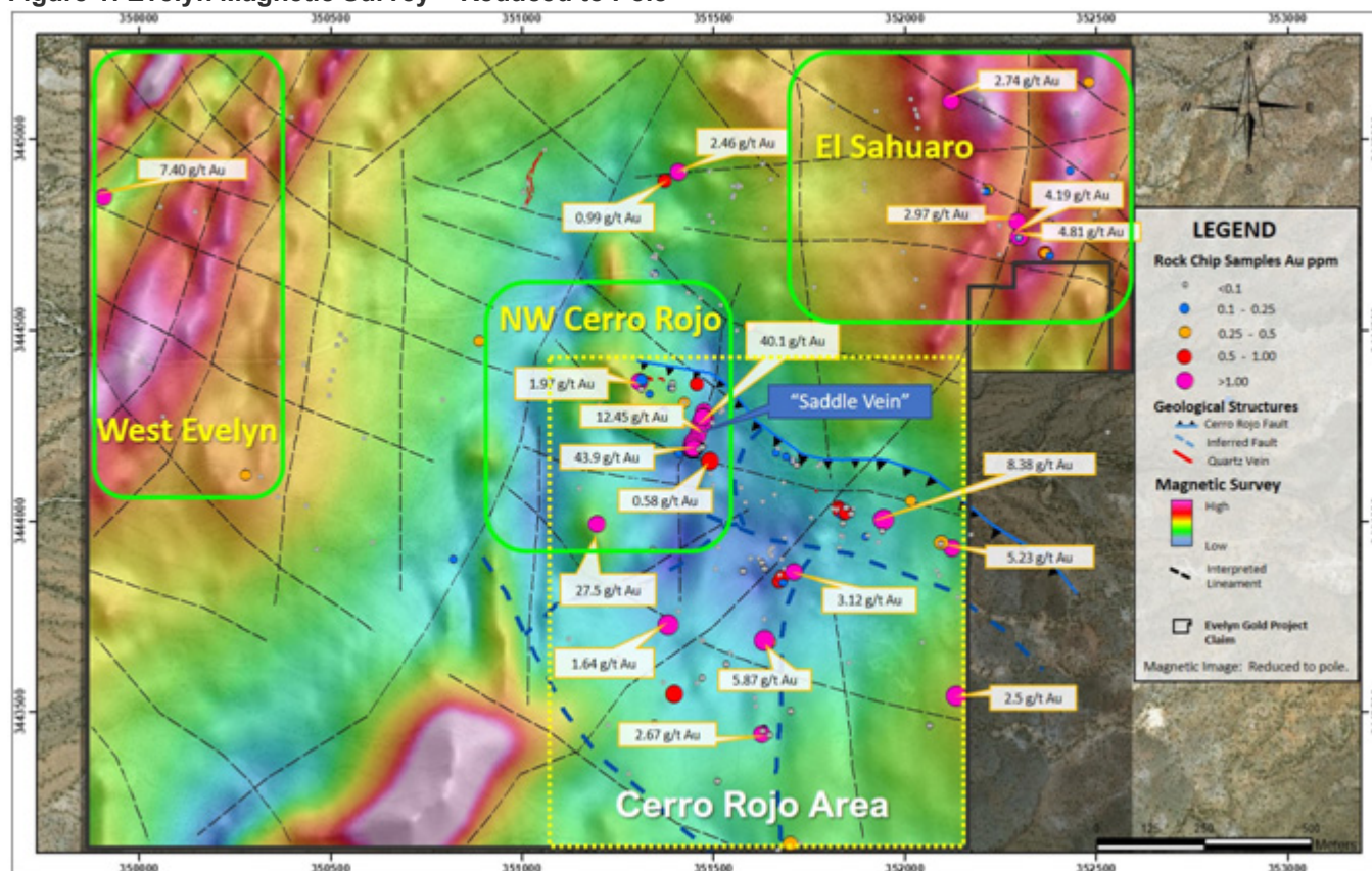
Figure 1: Evelyn Magnetic Survey – Reduced to Pole
