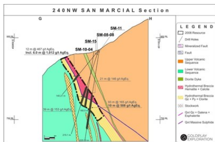
Figure 3: San Marcial Cross Section G-H (CNW Group/Goldplay Exploration Ltd)
